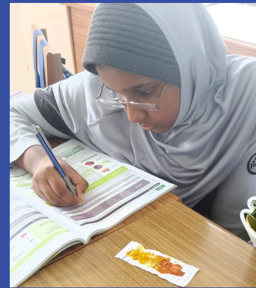
Testing Acids and Bases with turmeric
